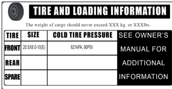
Tire and Loading Information Placard – Figure 1-1
